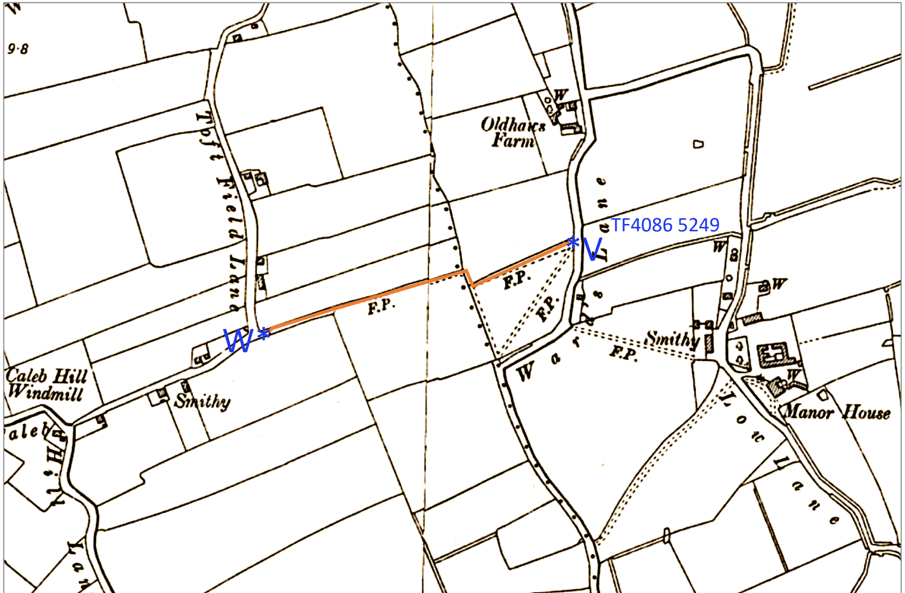
Wrangle Ward's Ln to Old Leake FP 1905 OS 6in Lincs 100.NE&101.NW at A4 size scale about 1:4730
