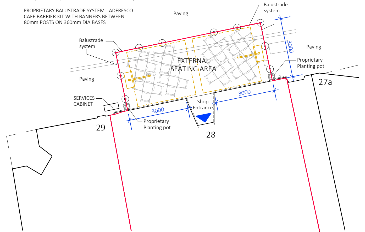
PROPOSED EXTERNAL SEATING AREA PLAN 1:100 0 1 2 3 4 5 6 7 8 9 10m
