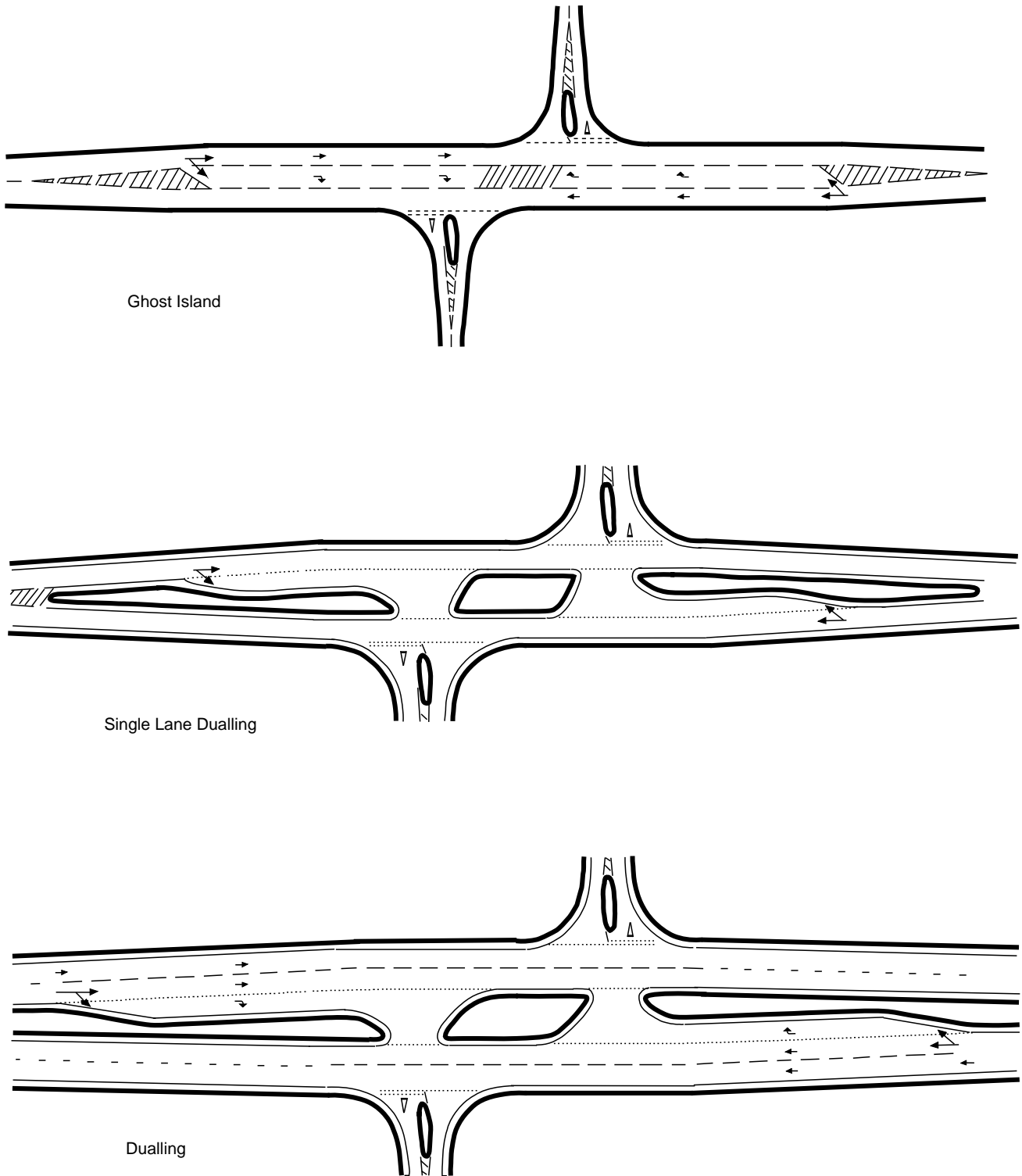
Figure 8/2 : Alternative Right / Left Staggered Junctions
