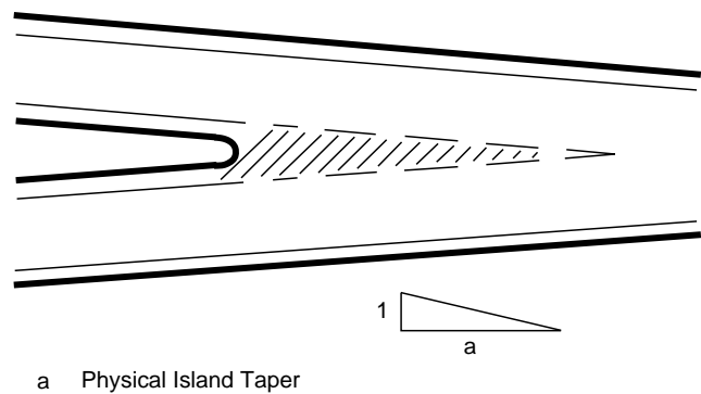
Figure 7/9 : Physical Island Development and Taper (para 7.30)
