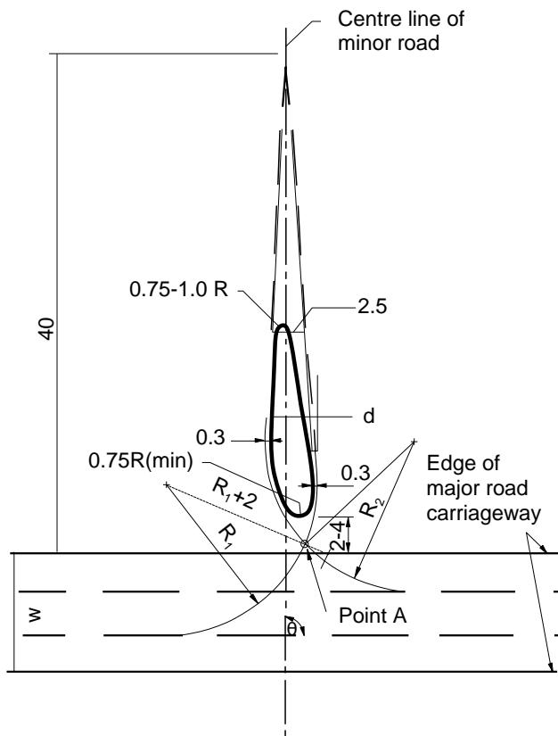
Figure A2/1: Design of Rural Channelising Island (Dimensions in metres)
