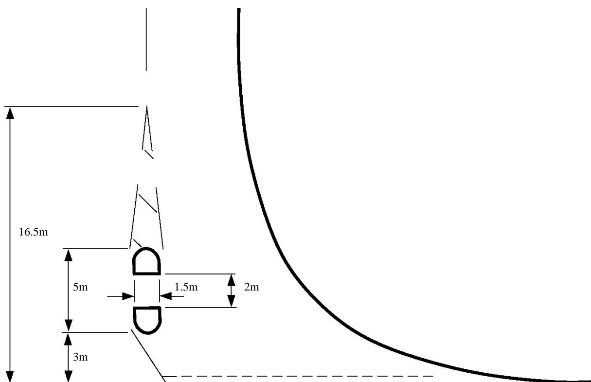
Figure 5/2: Typical Urban Separation Island (para 5.12)
